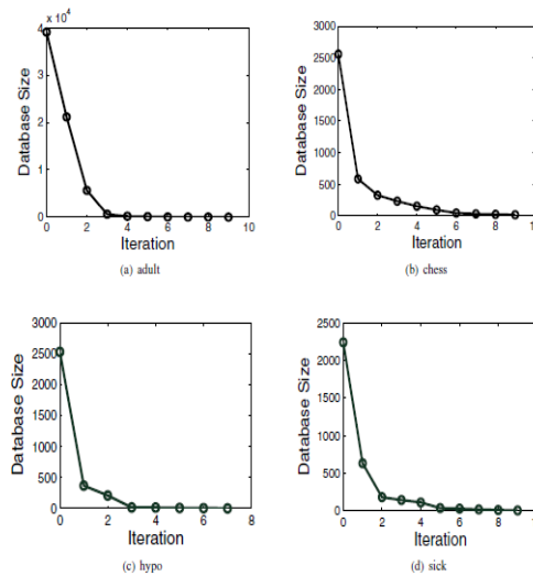
Fig. 3 Problem Size Reduction
