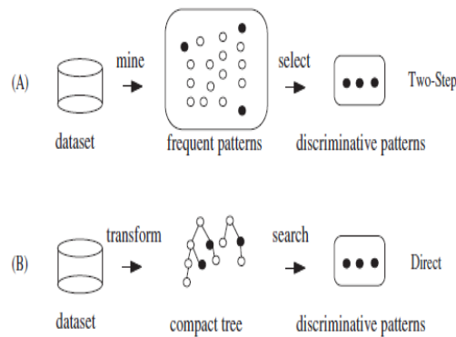
Fig. 1 Two step Vs DDPMine approach
